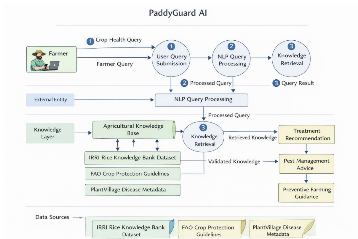
Figure 4.4: Data Flow Diagram of the PaddyGuard AI Advisory System
