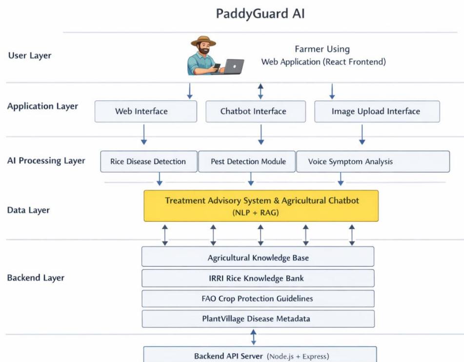
Figure 4.1: High-Level System Architecture of PaddyGuard AI
