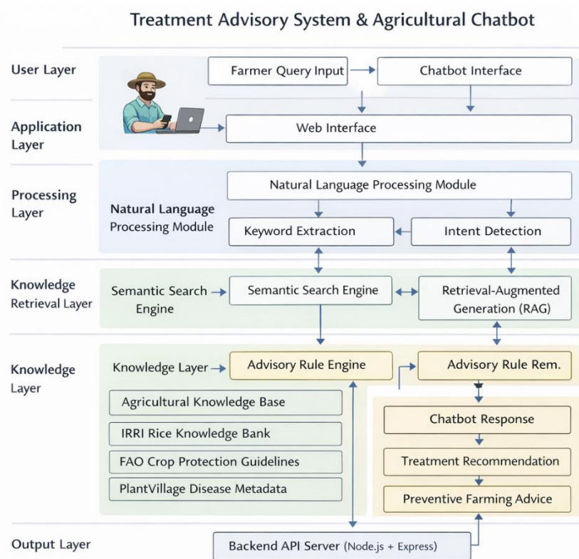
Figure 4.3: Architecture of the Treatment Advisory System and Agricultural Chatbot
