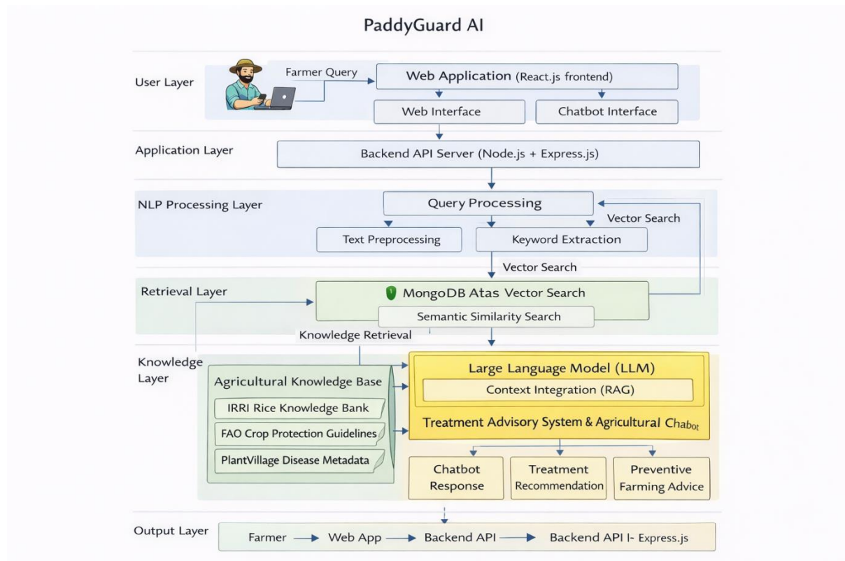
Figure 3.2: RAG Architecture of the PaddyGuard AI Advisory Chatbot
